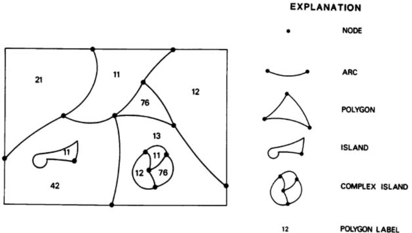
Figure 1.--Topological elements of a polygon map.
