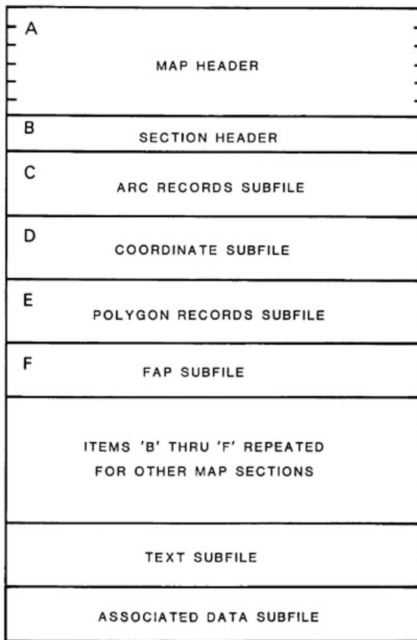
Figure 2.--GIRAS file structure.
