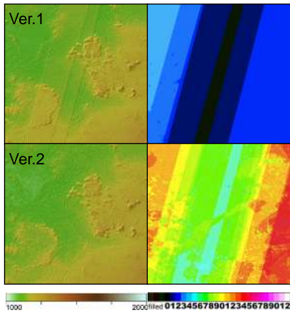
Figure 13 - Elevation and stacking in S31E023 (Southern Africa); GDEM1 above, GDEM2 below, elevation on the left, stacking number on the right.
