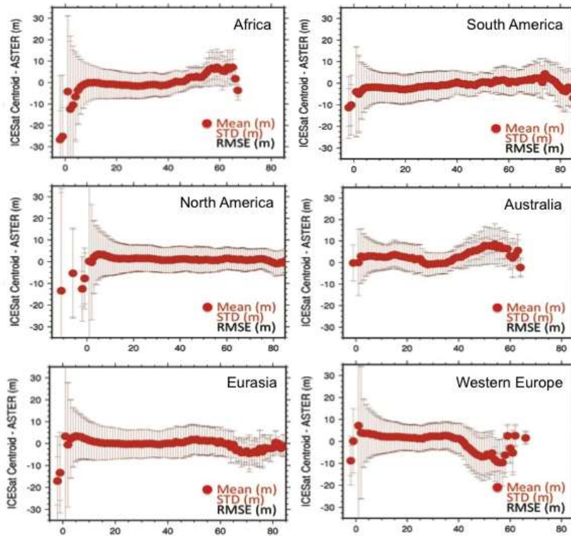
Figure 12 - ICESat - GDEM2 differences as a function of the number of ASTER scene pairs (“NUM”) used in generating elevations at a given pixel. Recall “NUM” < 0 corresponds to elevations filled from non-ASTER sources.
