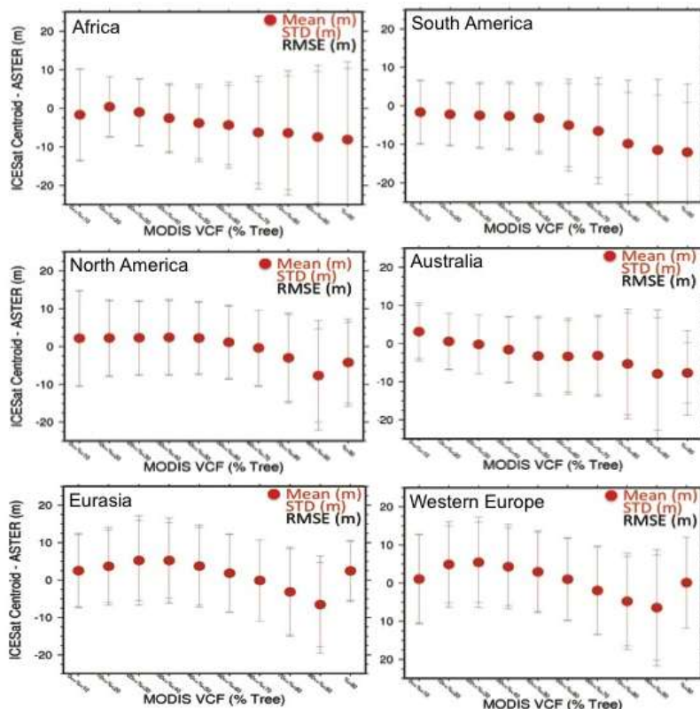
Figure 11 - GDEM2 differences as a function of VCF percent tree cover (increments in 10% cover from 0 to 100%).
