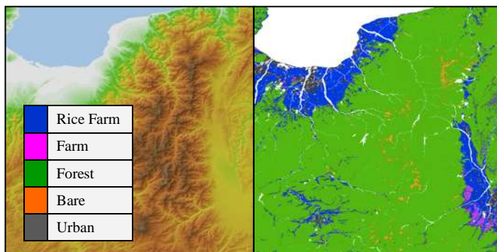
Figure 7 - The northwest GDEM2 tile of the 4-tile Japan study site (left), the GSI Land cover used in the study (right). See figure 1 to orient to the entire study area.
