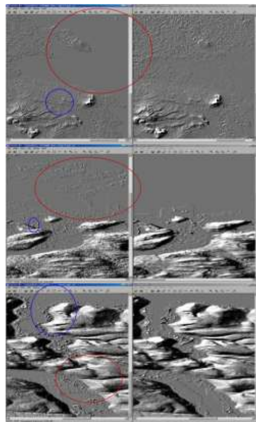
Figure 14 - Changes between GDEM1 (right) and GDEM2 (left) resulting from improvements in water masking. Top is Bolivia (tile s19w068), middle is Canada (tile n72w080), bottom is also Canada (tile n72w079).
